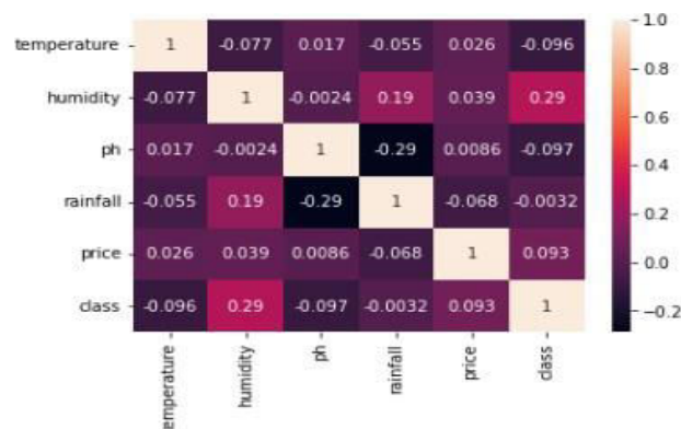
FIGURE. 4.2 FEATURE SELECTION
